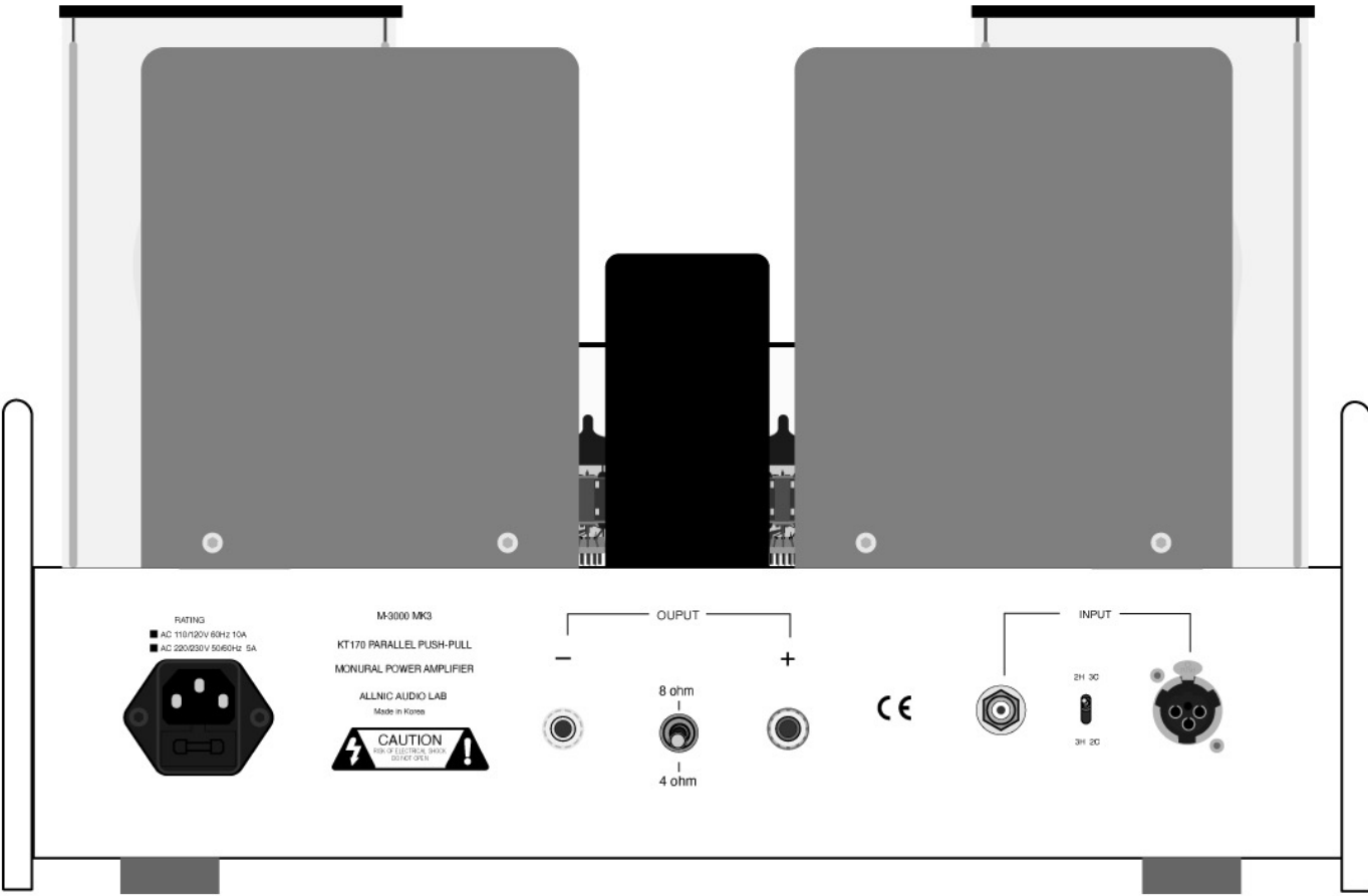
Figure 5 – Rear View
